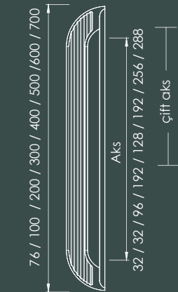
■ Alm. (L) LINE ALFA EKS.8040
