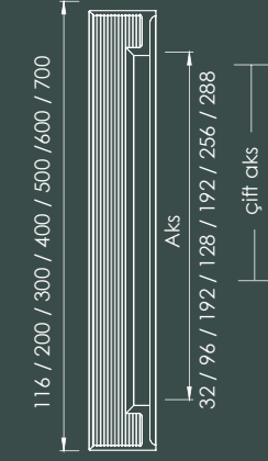
■ Alm. (L) LINE BETA EKS.8050
